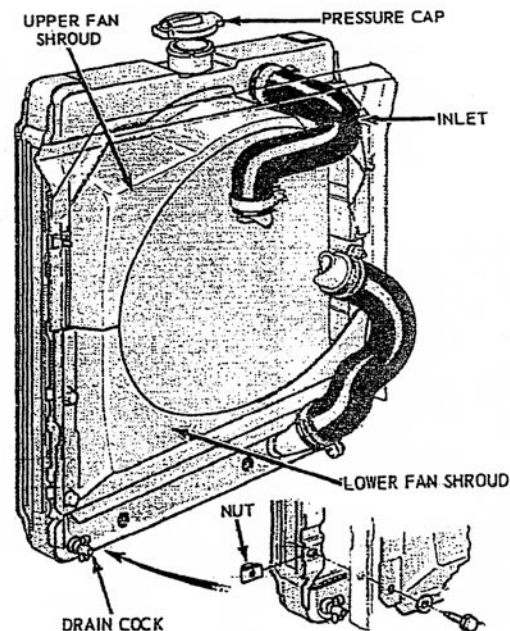
—240 Engine Radiator Installation—Typical
